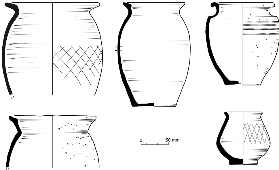
Fig 1: Examples of the most usual method of illustrating archaeological pottery, in elevation view with the left-hand side showing the section through the vessel, the right-hand showing the external view
