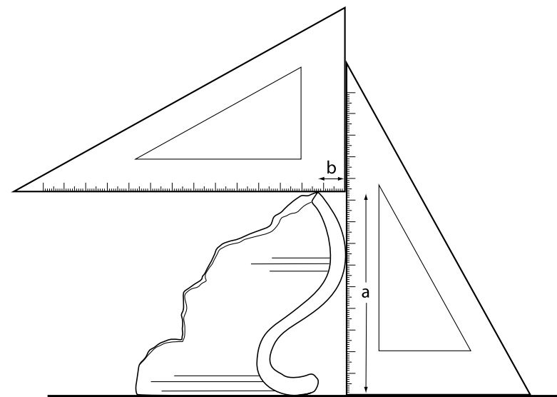
Fig 8: Measuring the height of a sherd
