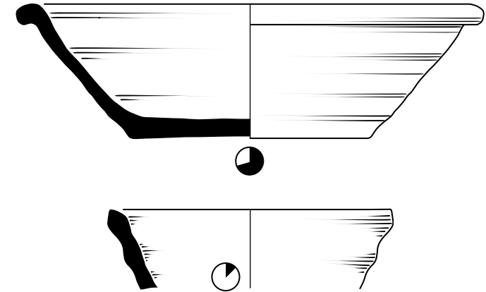
Fig 2: Small pie charts incorporated into the drawing indicate the proportion of the vessel present
