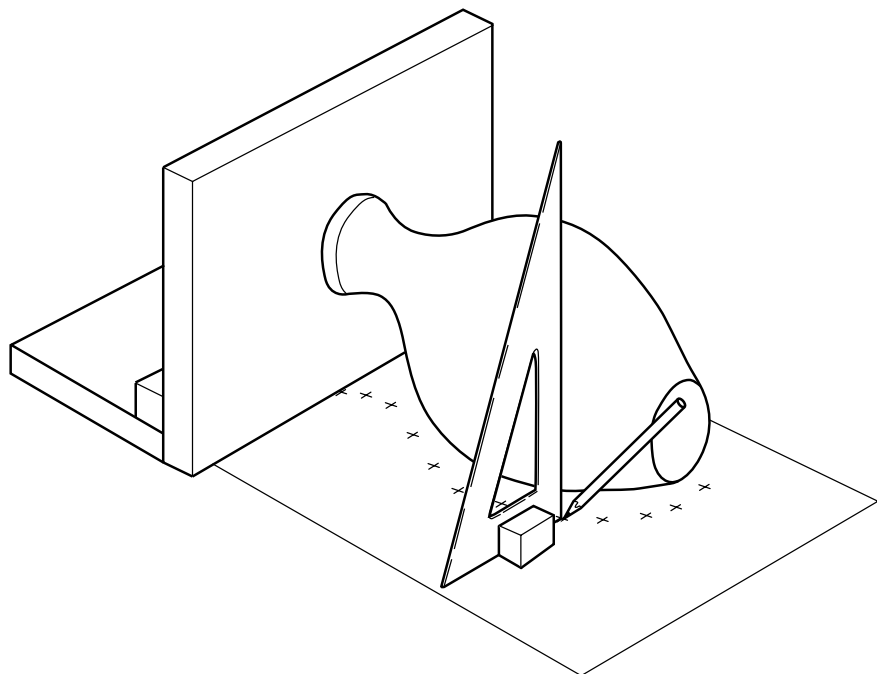
Fig 10: Alternative method of drawing the profile by resting the pot horizontally against a weighted backboard and directly sighting down and dropping points from the pot onto the drawing paper; (after Grinsell, Rahtz and Price Williams, 1974)
