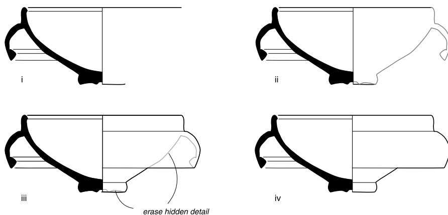
Fig 14: Transferring the profile to the right-hand (exterior) side and removing 'hidden' portions
